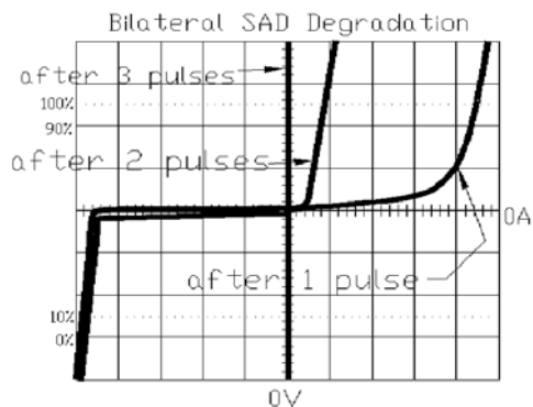
Figure 7 P6KE220CA SAD degradation under ~300mJ pulses. Note how only the reverse-biased junction degrades and fails because of its higher power dissipation. The clamp voltage drops as the device is stressed.
