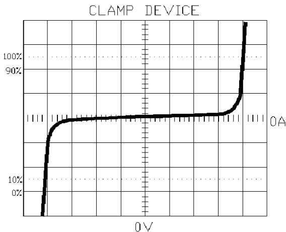
Figure 2 Clamp Device V-I characteristics. The voltage on the near- vertical portion of the curve is the clamp voltage.
