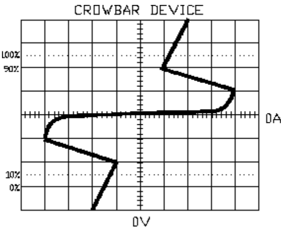
Figure 1 Crowbar Device Characteristic V-I Curve. The breakover voltage is that extreme where the curve begins to fold back. The voltage at the point at which it stops folding back is the turn-on voltage.
