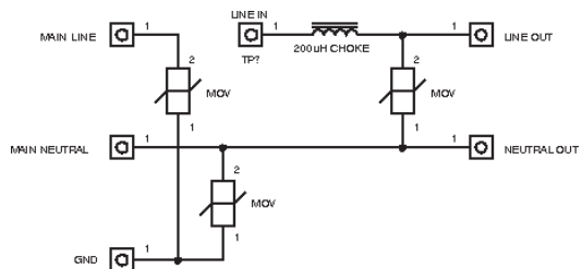
Figure 5 Line-Voltage “Hybrid” Suppressor
