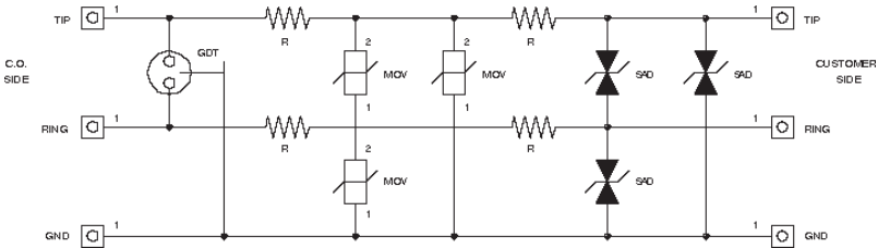
Figure 7 Telecom Surge Suppressor
