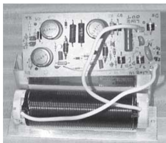
Photo 8 Open-frame Series-Mode Transient Suppressor
