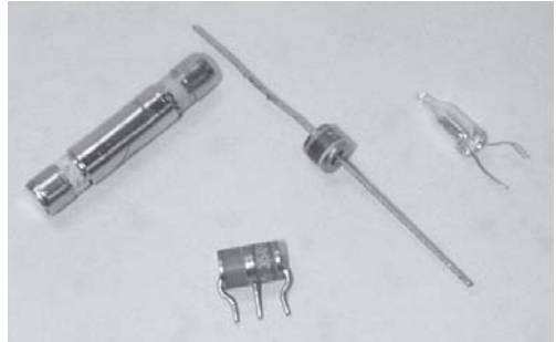
Photo 3 Gas Discharge Tubes
