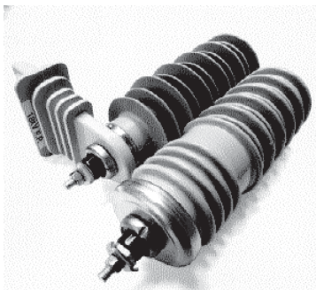
Photo 4 Varistors for Power Distribution Surge Protection.
