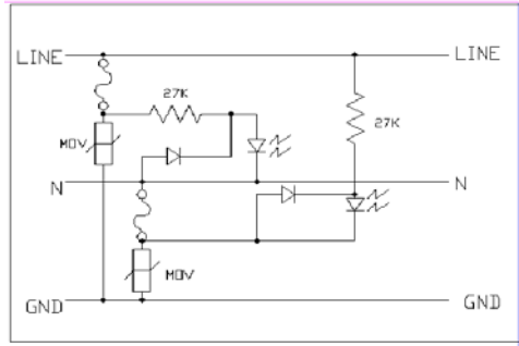
Figure 5 Typical MOV-based surge suppressor with LED indicator circuit. The indicator circuit prevents a low-current tester from reading the MOV clamp voltage because the LED circuit presents a much lower impedance than the MOV. In this case, a tester with at least 15\text{mA} of available current would be needed to test the 120\text{VAC} line voltage suppressor.
