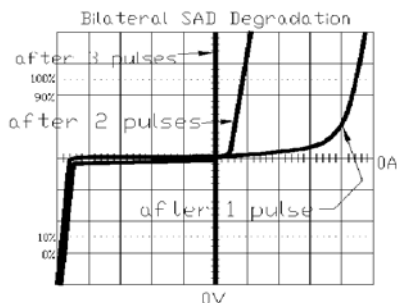
Figure 3 Bilateral SAD Degradation
