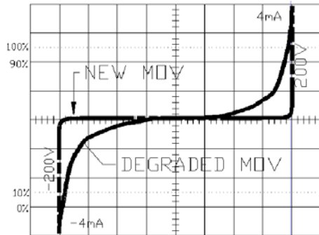
Figure 6 Thermal runaway characteristics in a small MOV.
