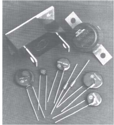
Photo 5 Metal-Oxide Varistors. These come in a wide variety of packages. Only a few are shown here.
