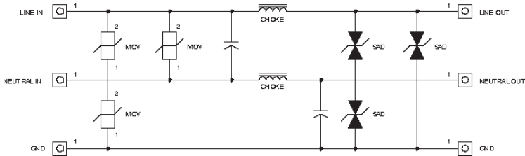
Figure 6 Line-Voltage Suppressor with MOVs, SADs, and RFI Filter
