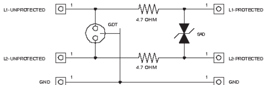
Figure 8 Data Line Suppressor
