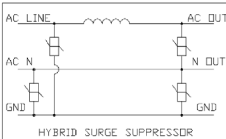
Figure 4 Typical hybrid suppressor with MOVs and choke inductor. There is an almost endless variety of suppressor circuit topologies, so adequate testing of a suppressor requires knowledge of the circuit.
